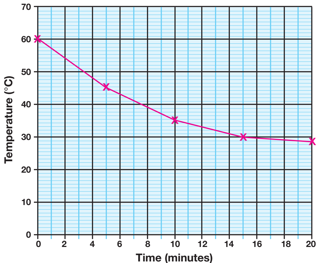
Cooling a hot drink using ice
