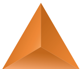
Triangular-based pyramid
