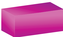
Cuboid
