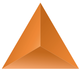
Triangular-based pyramid
