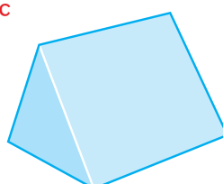
triangular prism
