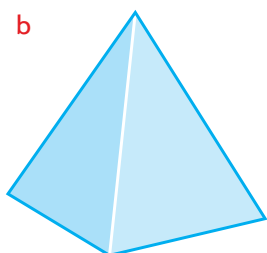
square-based pyramid
