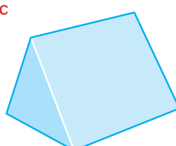
triangular prism
