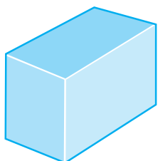
cuboid
